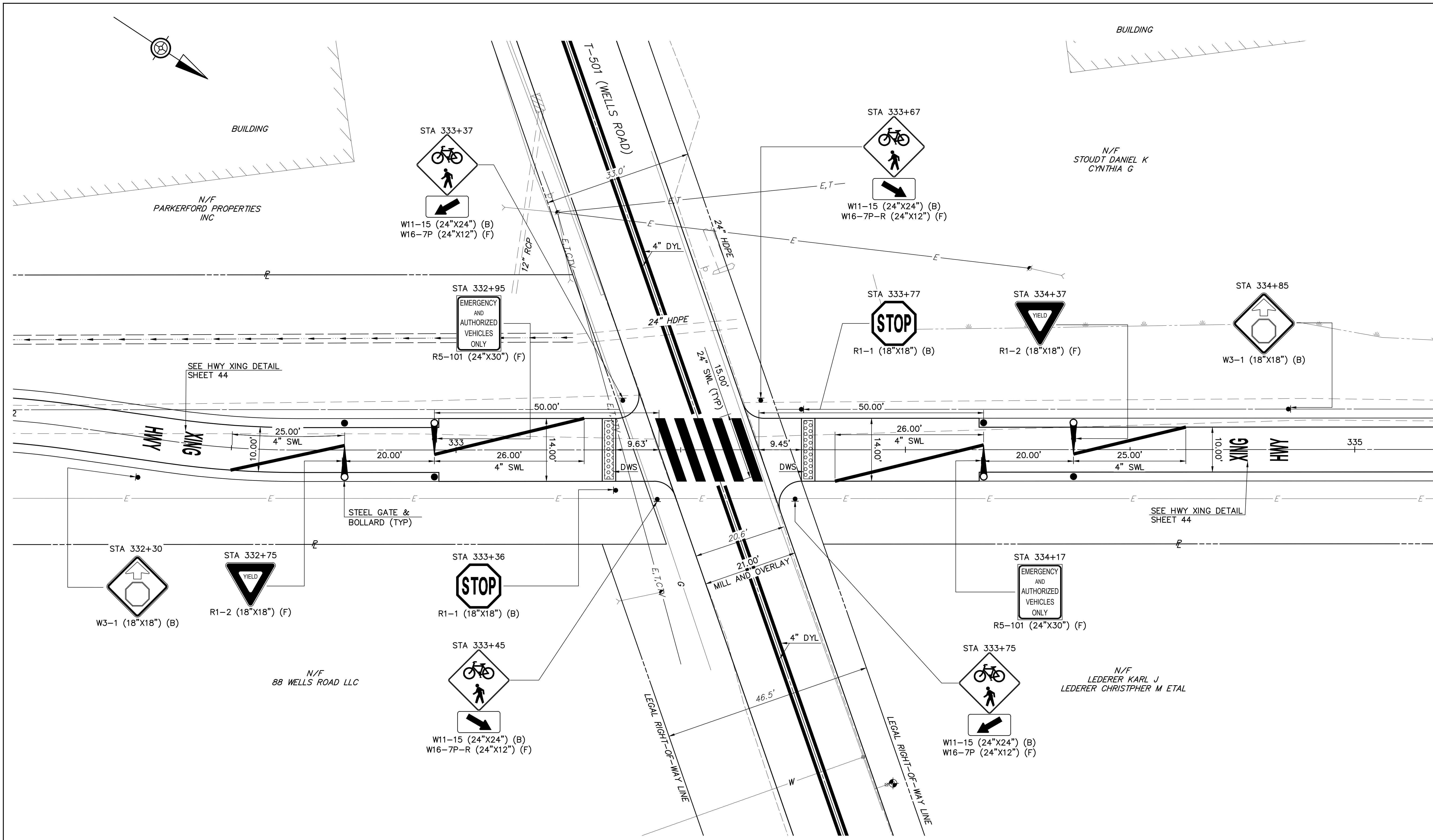
TYPICAL CROSSING PLAN
